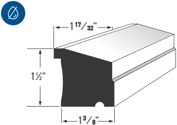
SUB SILL NOSE AZM-6933 LENGTH: 16'
