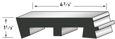
SILL AZM-948 LENGTH: 16'
