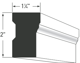
BRICK MOULD AZM-180 LENGTHS: 16' | 17' | 18''
