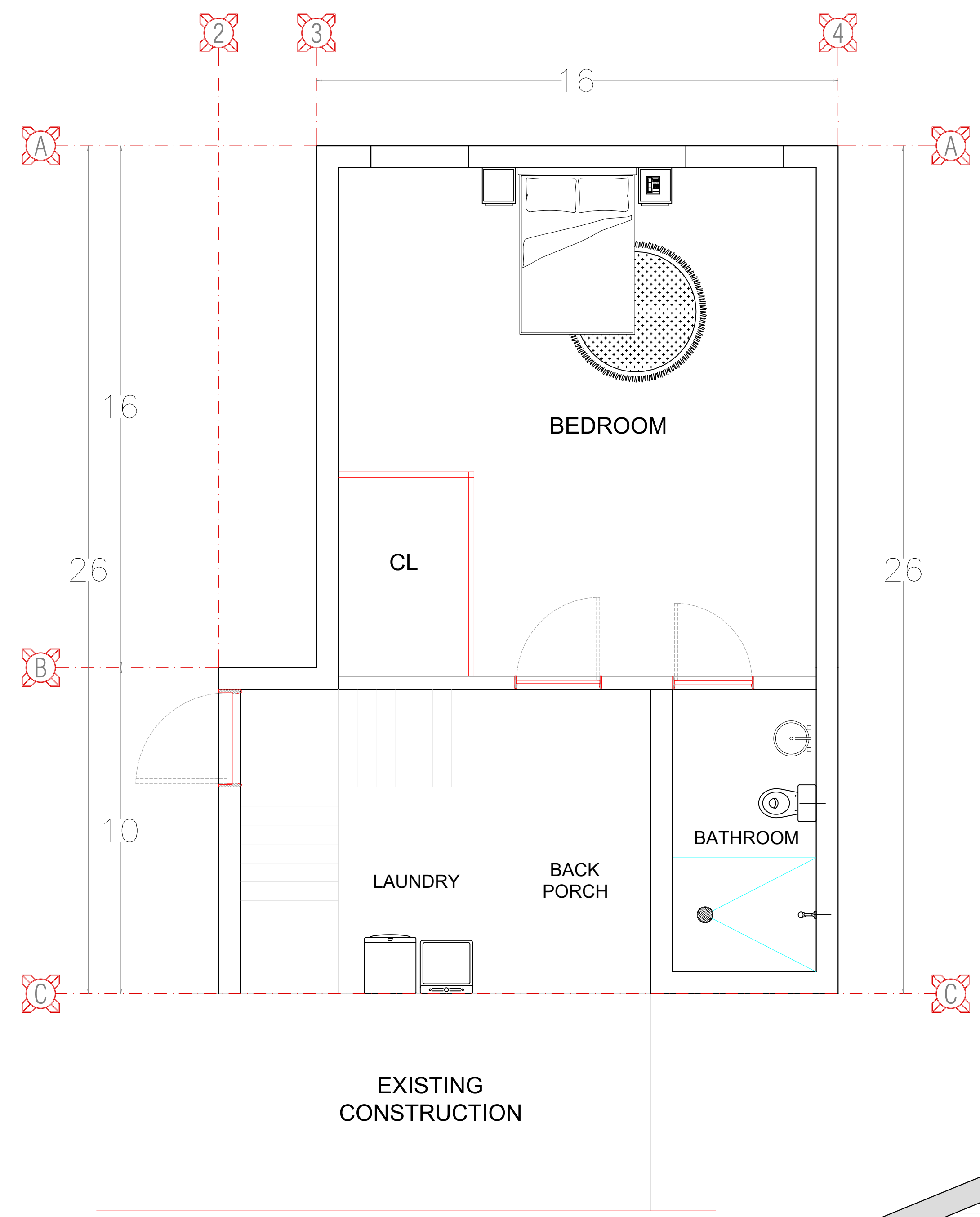
FLOOR PLAN ESC 1:50 [ft]
